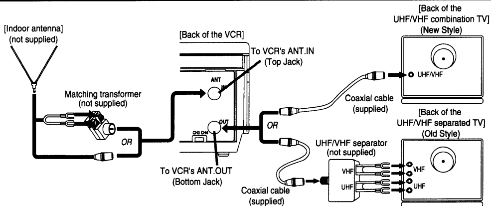
Fig.1: Indoor Antenna
