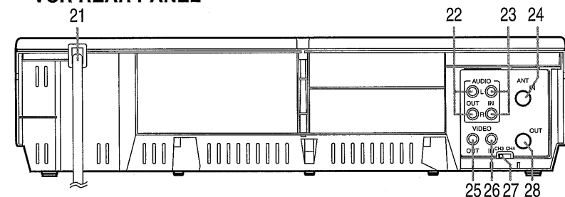
— VCR REAR PANEL —
