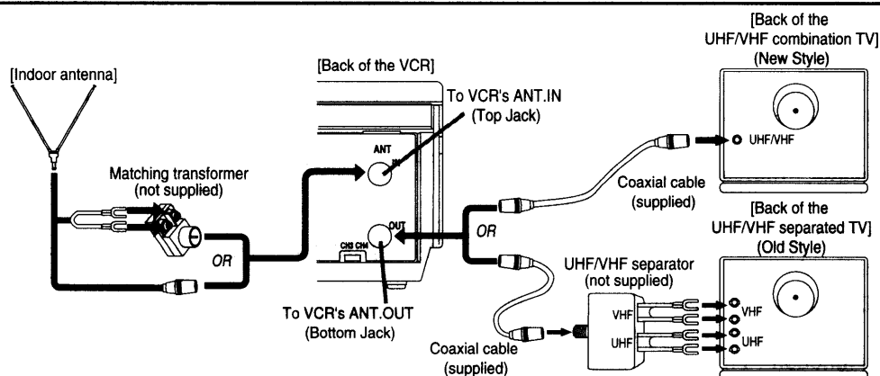
Fig.1: Indoor Antenna
