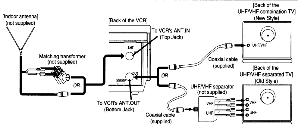
Fig.1: Indoor Antenna
